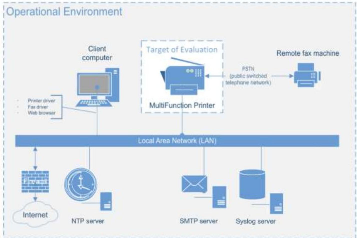
Figure 1: TOE Architecture
